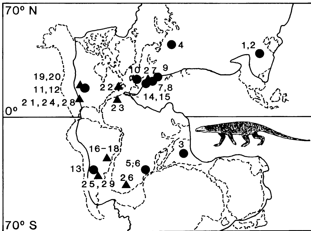
TEXT-FIG. 2. The distribution of raiusuchians plotted on a palaeogeographic map for the Triassic (Cox 1974). The modern continental outlines are shown with dashed lines, and the outlines of the Triassic supercontinent Pangaea are shown with a solid line. ● = Lower and Middle Triassic raiusuchians. ▲ = Upper Triassic raiusuchians. The numbers correspond to the twenty-nine genera of raiusuchians listed in Table 1.
